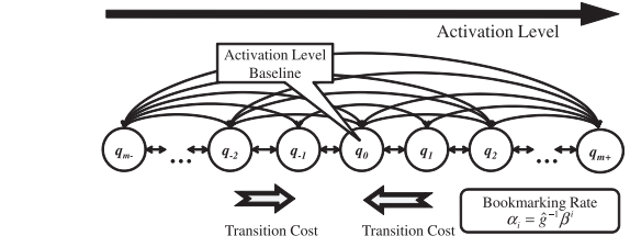
Fig. 9 A model of activation levels in SBM.
