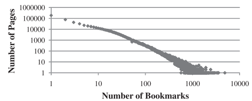
Fig. 2 Numbers of bookmarks.
