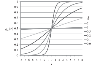
Fig. 14 Sigmoid function.
