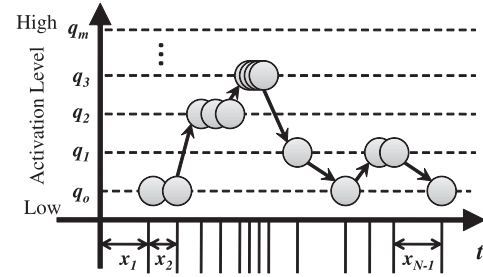
Fig. 8 Activation level based on arrival gaps.
