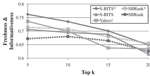
Fig. 17 Freshness and informativeness.
