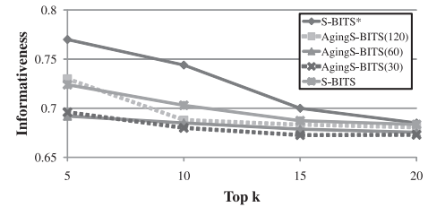
Fig. 20 Informativeness comparison among 3 types of S-BITS.
